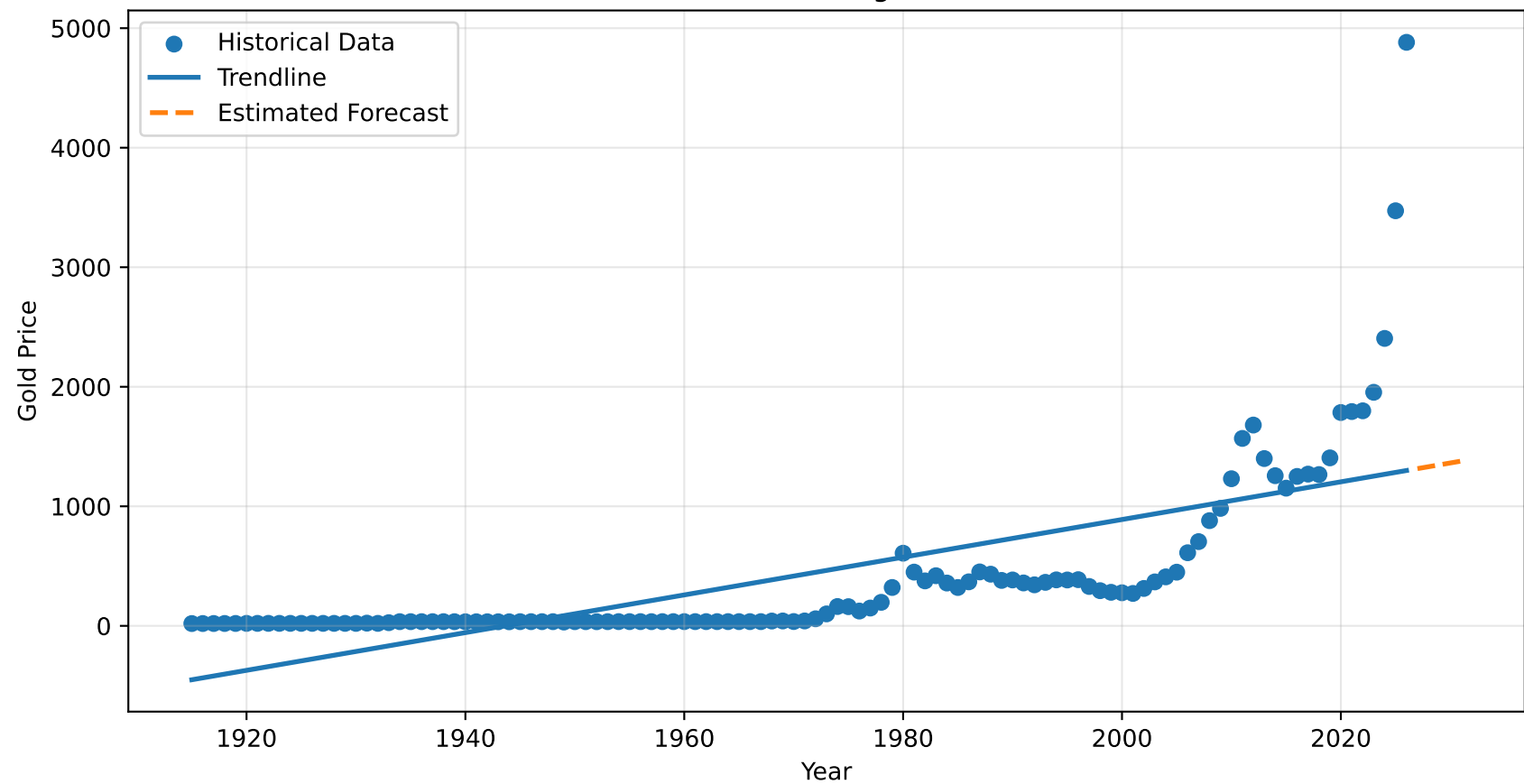
Gold Price Forecast Using Linear Trendline
